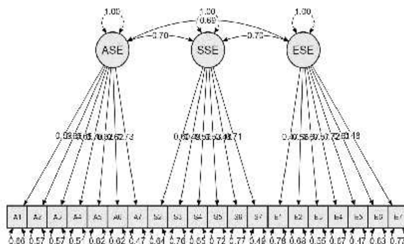
Figure 1. CFA Path Diagram on SEQ-C Model 2 (n = 278)
