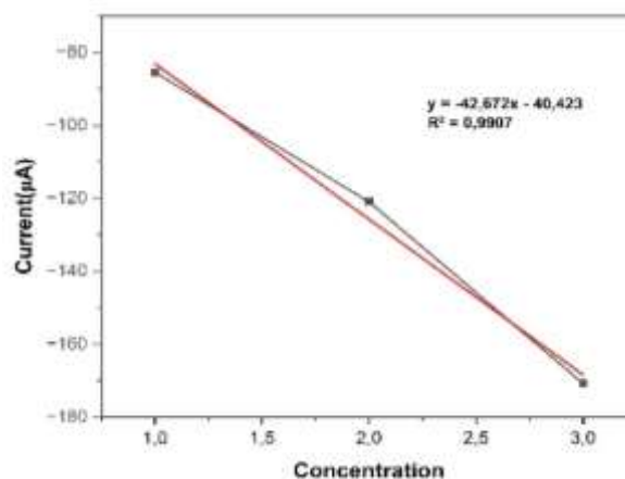
Figure 4. Calibration curve of \text{Zn}^{2+} using \text{NiAl}_2\text{O}_4 -modified GCE in 0.1 M KCl.
