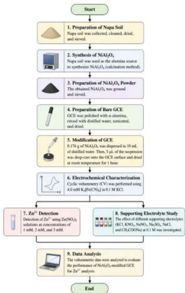
Figure 1. Research flow diagram of \text{NiAl}_2\text{O}_4 -modified GCE preparation and \text{Zn}^{2+} analysis.
