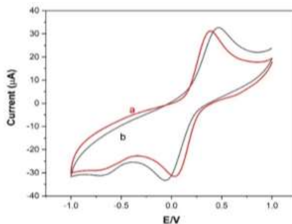
Figure 2. Cyclic voltammograms of (a) bare GCE and (b) \text{NiAl}_2\text{O}_4 -modified GCE in 4.0 mM \text{K}_3[\text{Fe}(\text{CN})_6] containing 0.1 M KCl at a scan rate of 100 \text{ mV s}^{-1} .
