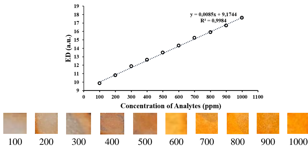
Figure 5. Sensor Standard Curve
