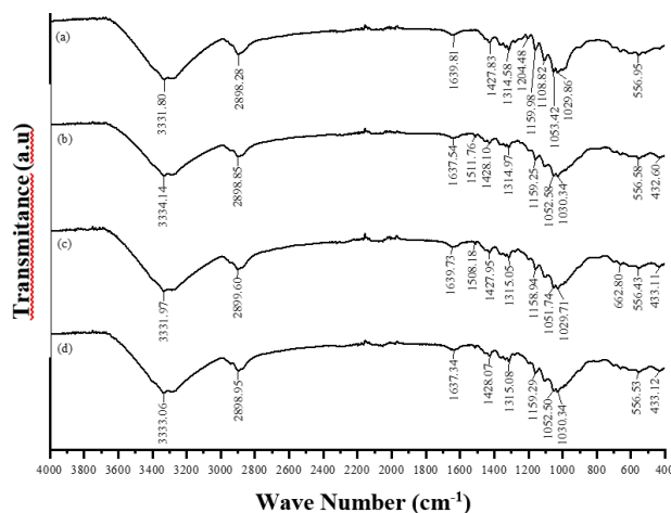
Figure 7. IR spectra of the censorship stage (a) Blank filter paper, (b) xerogel coated filter paper, (c) after censoring with \text{SCN}^- 0,01 and (d) after censoring with \text{SCN}^- 0,1.
